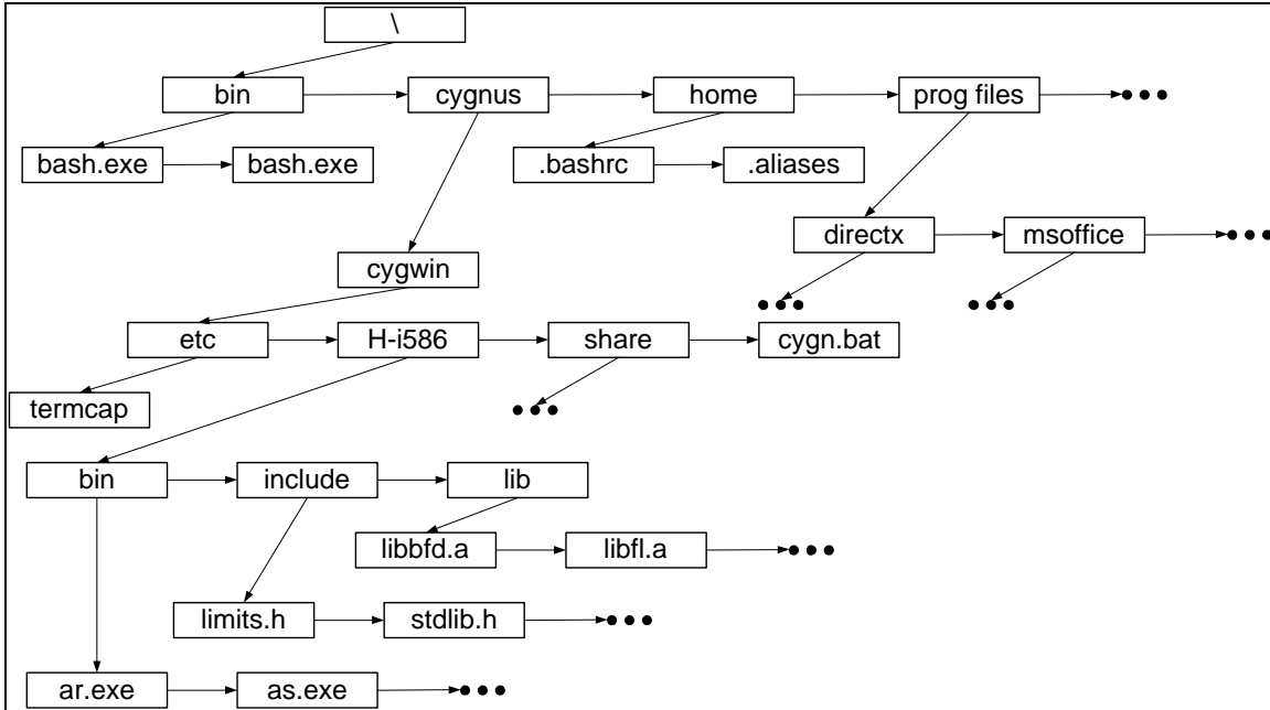
Figure 10-5 A Disk Directory Structure
