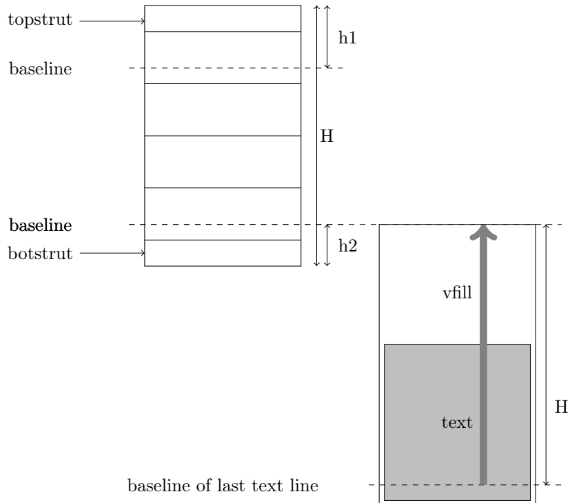
Figure 6: Case \langle n\text{rows} \rangle < 0 , \langle v\text{pos} \rangle = [b]
